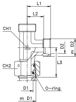
Type: 6046...1 Body
