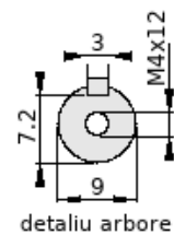
detaliu arbore
