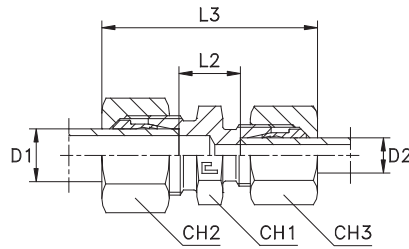
Type: 1041.. B3 Ring
