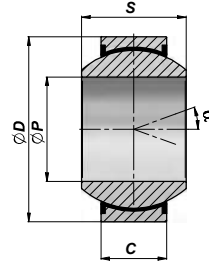
TYPE FW...2RS
