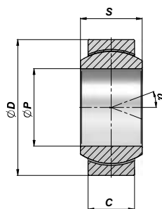
TYPE UK
