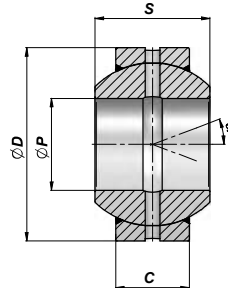
TYPE FO...2RS
