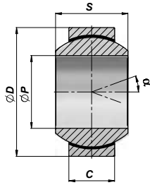
TYPE FW
