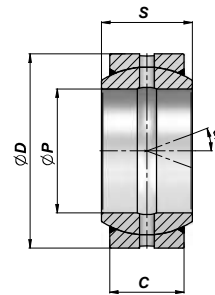
TYPE DO...2RS
