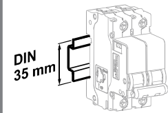
Installed on 35mm standard guide rail
