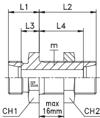
Type: 1036...1 Body
