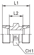
Type: 1035...1 Body
