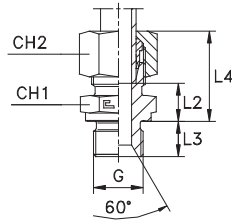
Type: 1003... B3 Ring
