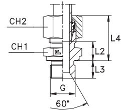
Type: 1003...4 B4 Ring
